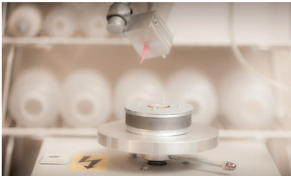
A fully-automated glue machine designed and constructed to fulfil the high requirements for a sample build.
