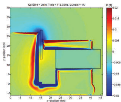
Simulated AC changes of the B-field.
