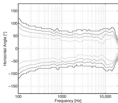
Fig. 9 Directivity of the Beolab 90 in Narrow-Front mode. Contours are in steps of 3 dB related to the on-axis response.
