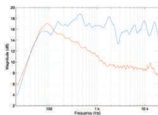
Fig. 3 On-axis frequency response (blue) and power response (red curve) of the BeoLab 5.
