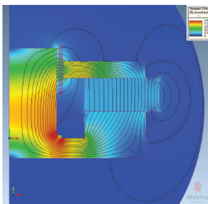
Flux lines and B field simulated in MagNet.
