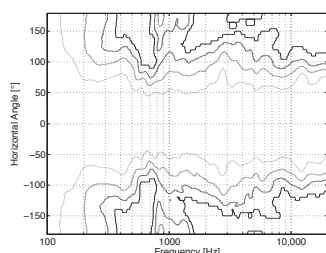
Fig. 2 Directivity of the BeoLab 5. Contours are in steps of 3 dB related to the on-axis response.
