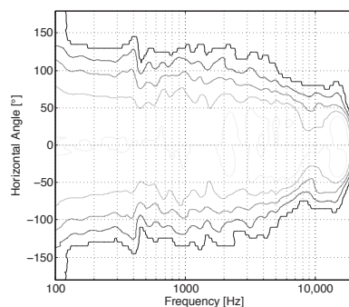
Fig. 10 Directivity of the Beolab 90 in Wide-Front mode. Contours are in steps of 3 dB related to the on-axis response.
