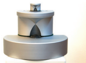
Fig. 1 The second prototype of the Acoustic Lens, which showed that a curved face was necessary to reduce comb filtering effects caused by edge diffraction.
