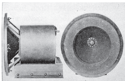
The Rice-Kellogg speaker unit based on the AIEE paper (1925). Source: www.aes.org
