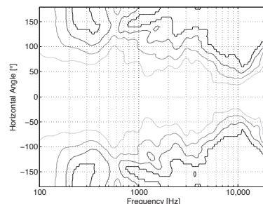
Fig. 8 Directivity of the BeoLab 90 with Beam Width Control disabled (only the front-centre woofer, midrange and tweeter operational). Contours are in steps of 3 dB related to the on-axis response.
